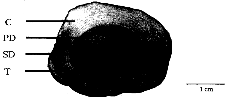
Figure 12. Enlarged and enhanced photograph of a cross-section of a walrus tooth showing cementum (C), transition ring (T), and primary dentine (PD). This tooth also shows a small area of apparent secondary dentine (SD). Note the presence of concentric rings in the exceptionally thick cementum.
